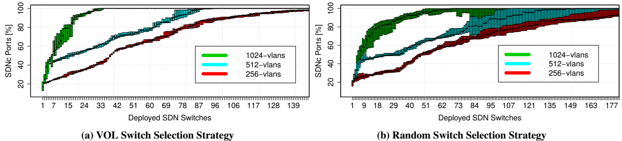
Figure 5: Percentage of SDNc ports as a function of deployed SDN switches, under different VLAN availability. When more VLANs are supported by legacy devices, more SDNc ports can be realized with fewer SDN switches.
