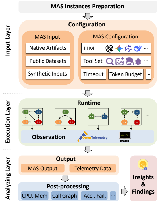
Figure 1: MAESTRO architecture overview.
