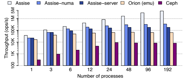
Figure 10: Scalability of atomic 4KB file operations. Log scale.
